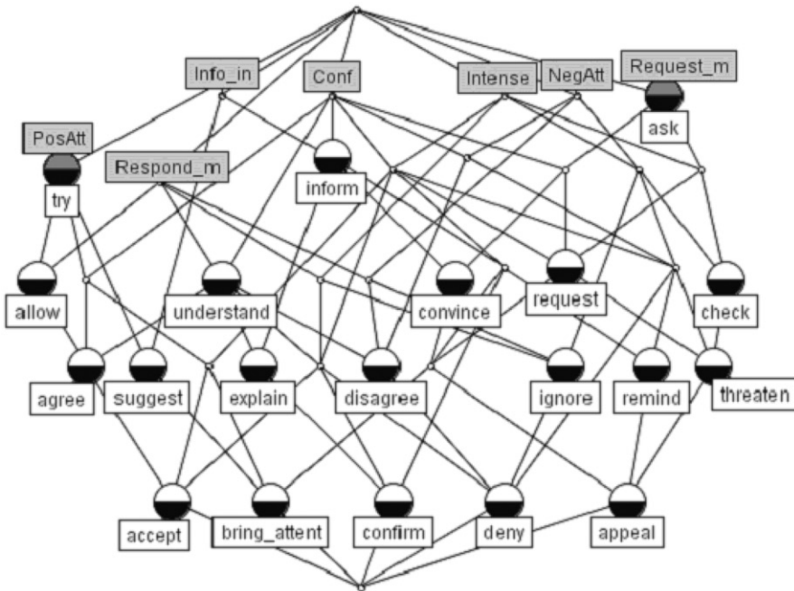
Figure 4. The concept lattice for communicative actions. Each communicative action has a unique set of attributes.
