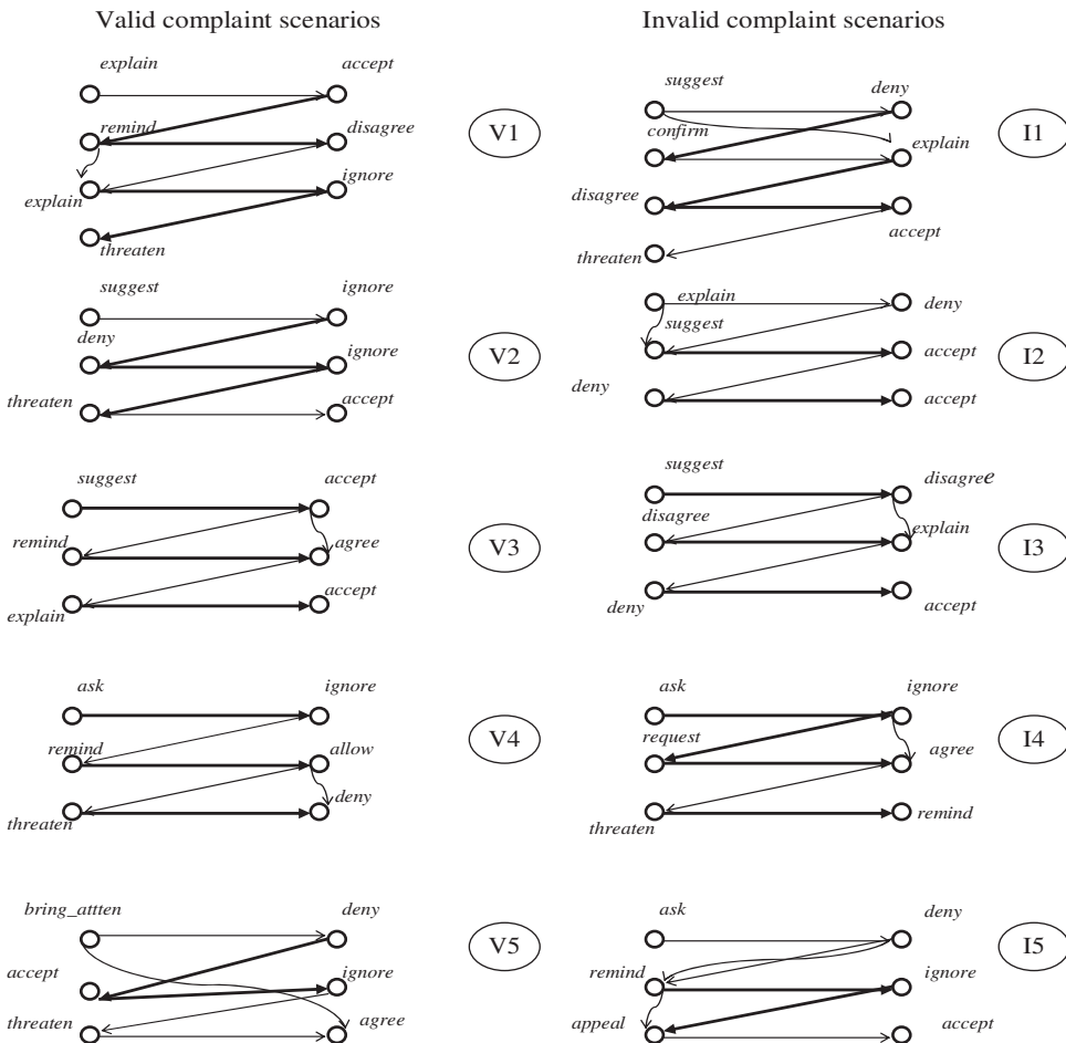
Figure 5. The training set of scenarios.
