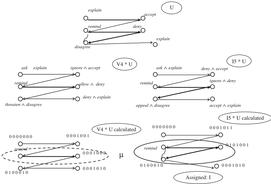
Figure 6. A scenario with unassigned complaint status and the procedure of relating this scenario to a class.
