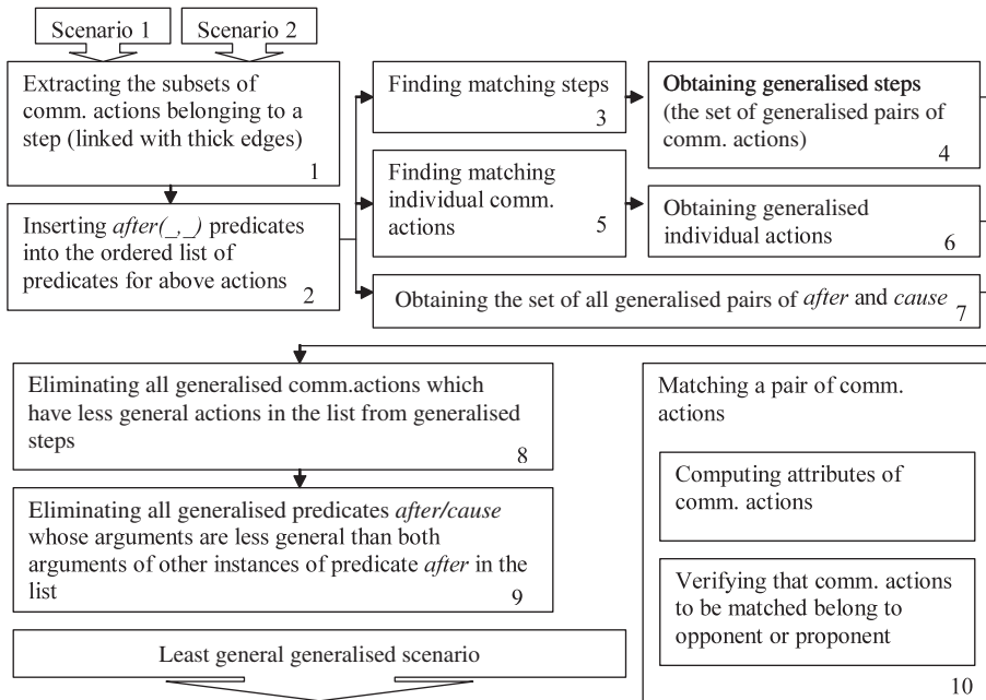
Figure 11. The chart of the algorithm for finding similarity between scenarios.
