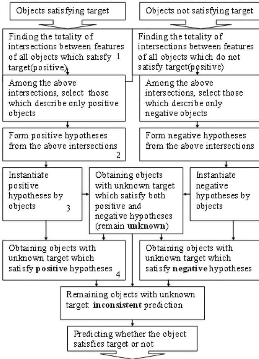
Figure 8. The chart for reasoning procedure of Jasmine . Note that the prediction schema is oriented to discover which mental actions/attitudes cause the target and how they do it, rather than just searching for common features for the target which would be much simpler (six units on the top). The respective clauses (1–4) are spelled out below, and sample results for each numbered unit (1–4) are presented in Figure 9.
