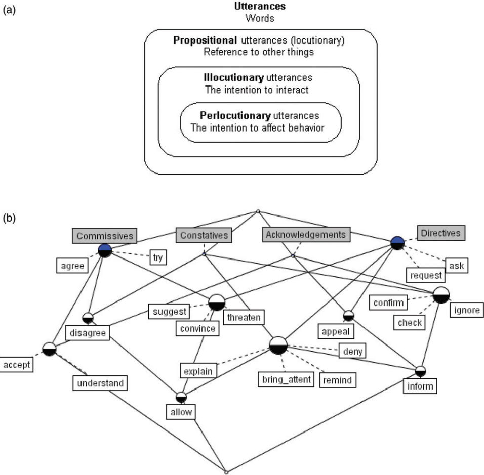
Figure 2. (a) Categories of speech acts. (b) The concept lattice for communicative actions adapting speech act theory to our domain. Each communicative action does not have a unique set of attributes: calculation of similarity might be inadequate.
